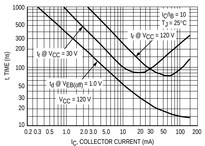
Figure 8. Turn-On Time
