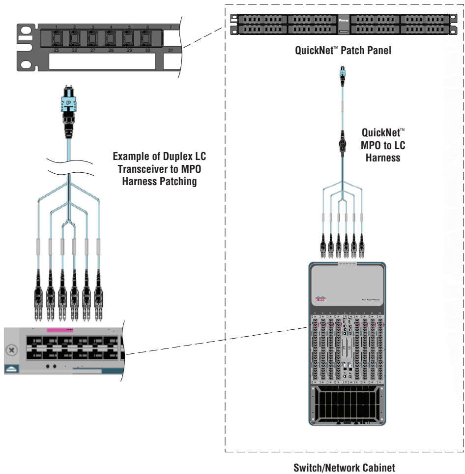
Figure 5 – Switch Port Equipment Harnesses
