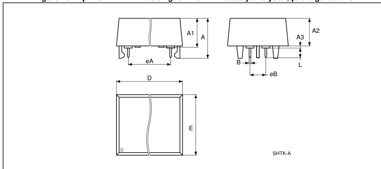
Figure 23. 4-pin SNAPHAT® housing for 120 mAh battery &amp; crystal, package outline
