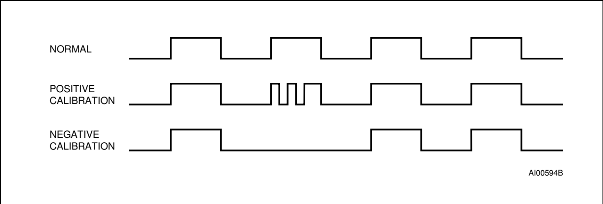
Figure 14. Calibration waveform
