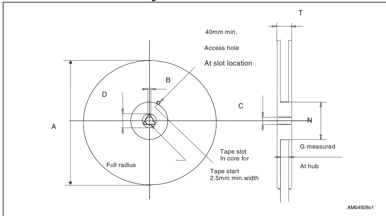
Figure 26. Reel schematic
