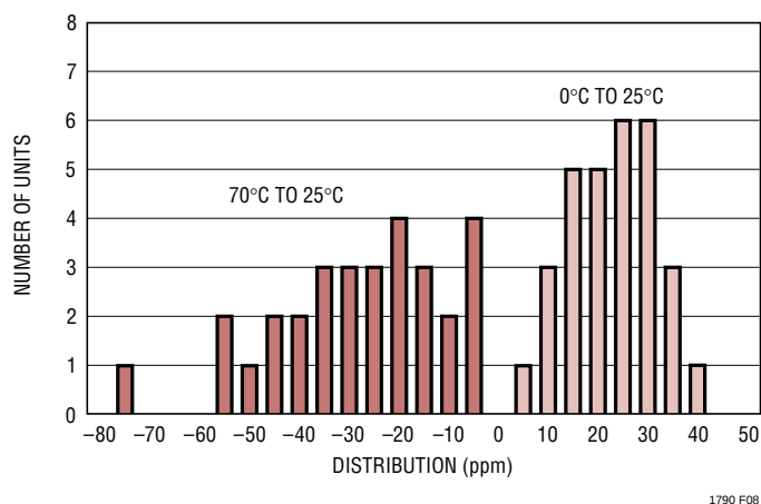
Figure 8. Worst-Case 0°C to 70°C Hysteresis on 30 Units
