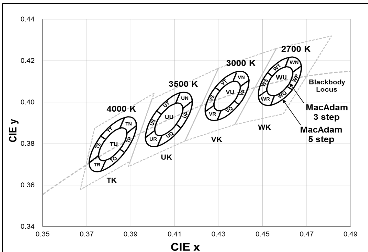
e) Chromaticity Region & Coordinates ( I_F = 150 \text{ mA} , T_s = 85^\circ \text{C} ) : "K" (Kitting for MacAdam 3-step)
