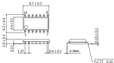
SOP14
