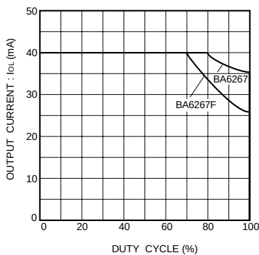
Fig.4 Output conditions
