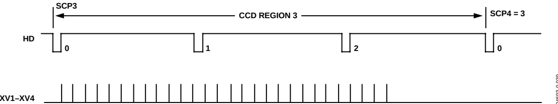
Figure 38. Sweep Mode Timing Example with SVREP_MODE = 2 and SVREP3 = 28
