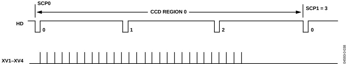
Figure 37. Sweep Mode Timing Example with SVREP_MODE = 1 and SVREP0 = 28
