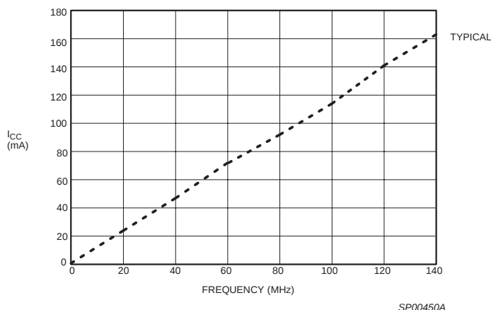
Figure 5: V_{CC} vs. Frequency at V_{CC} = 5.0V , 25^{\circ}C
