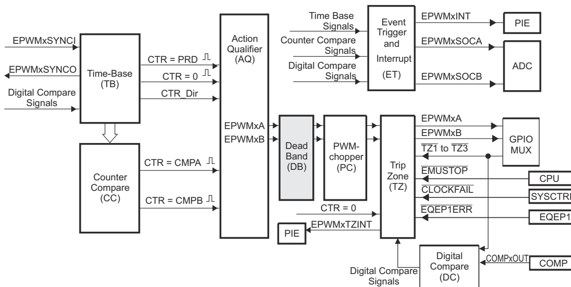
Figure 3-28. Dead-Band Submodule
