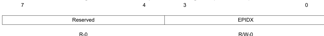
Figure 17-15. USB Endpoint Index Register (USBEPIDX)
