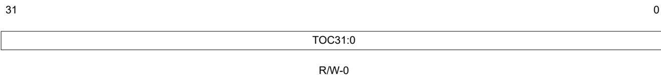
Figure 16-35. Time-Out Control Register (CANTOC)
