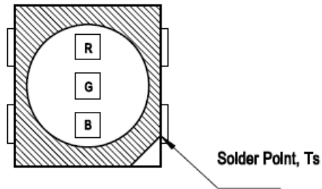
Figure 17: Solder Point Temperature on PCB
