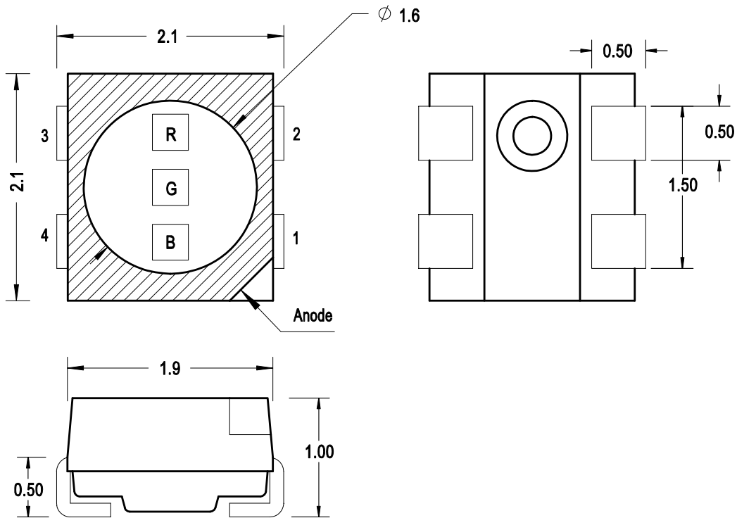
Figure 1: Package Drawing
