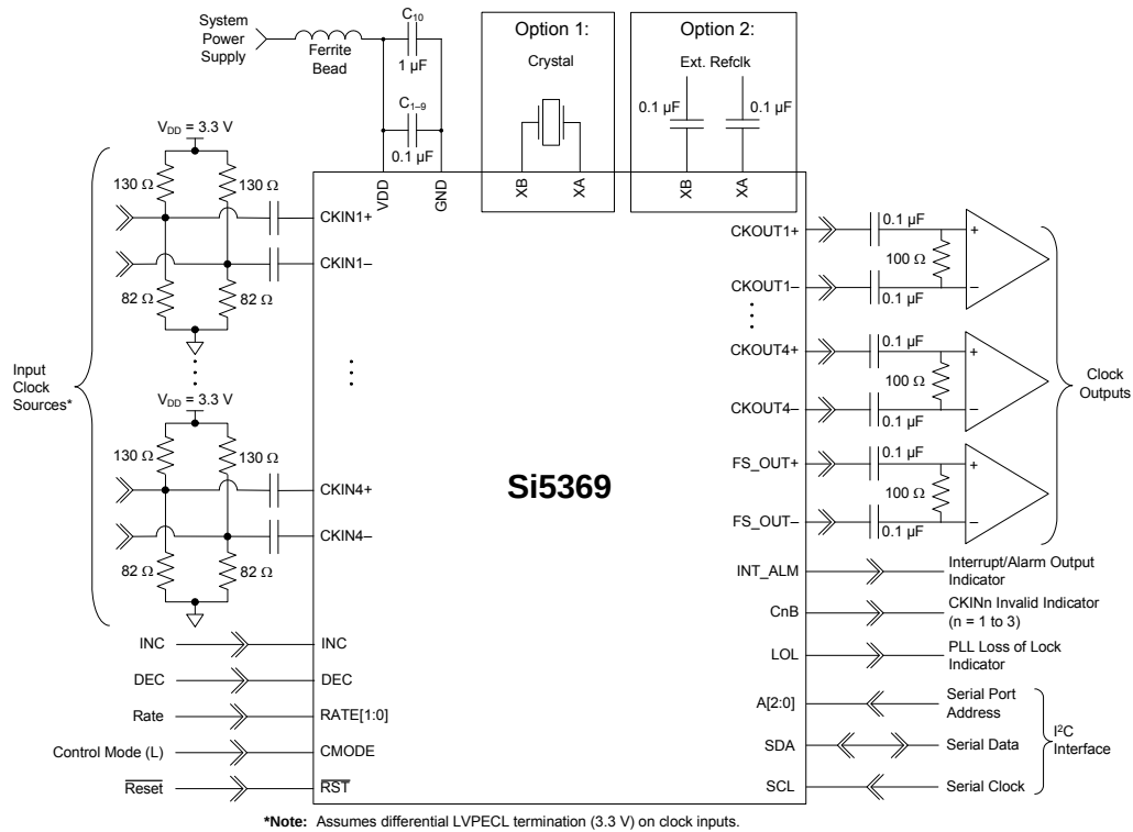
Figure 7. Si5369 Typical Application Circuit (I²C Control Mode)
