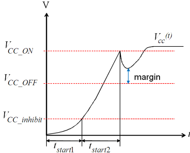
Figure 65. The V_{\text{CC}} at start-up is made of two segments given the short-circuit protection implemented on the HV source
