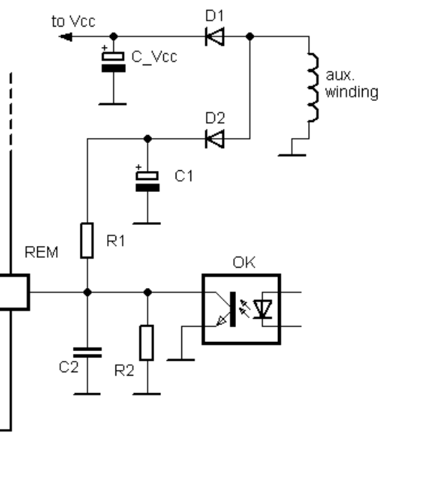
Program of Remote Control Input
