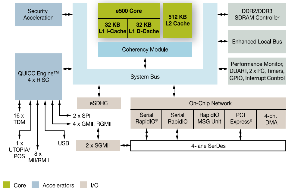
MPC8569E Block Diagram
