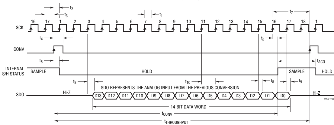
LTC2355-14 Timing Diagram
