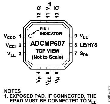
Figure 4. ADCMP607 Pin Configuration
