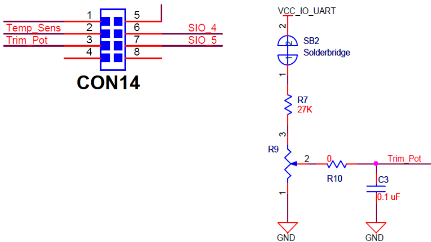
Figure 11: Trim Potentiometer
