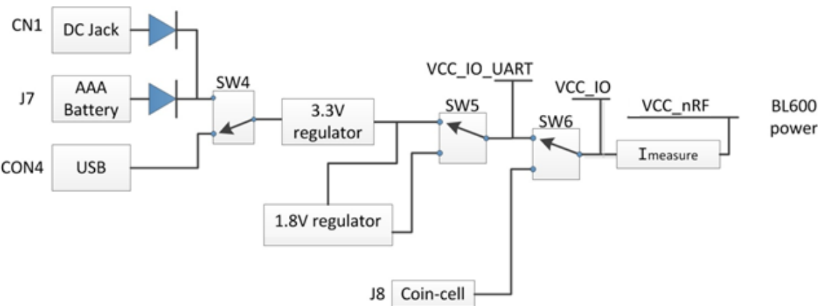
Figure 3: BL600 power supply
