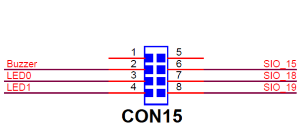
Figure 9: Buzzer
