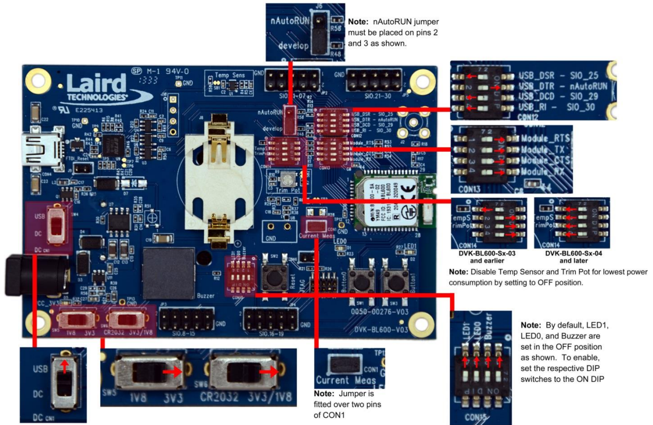
Figure 2: Correct development board settings
