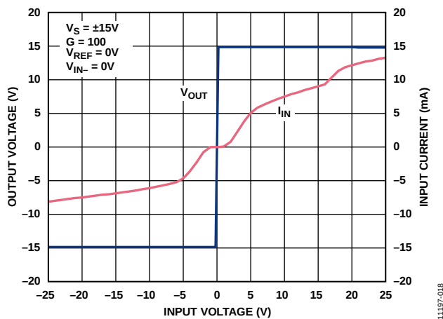
Figure 17. Input Overvoltage Performance; G = 100 , V_S = \pm 15V
