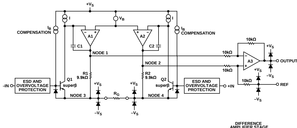
Figure 55. Simplified Schematic
