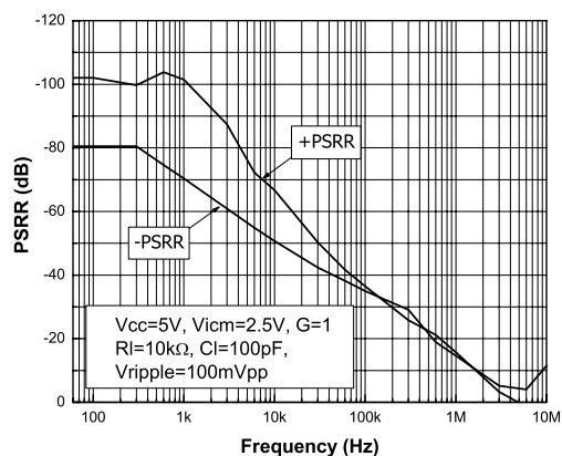
Figure 45. PSRR vs. frequency
