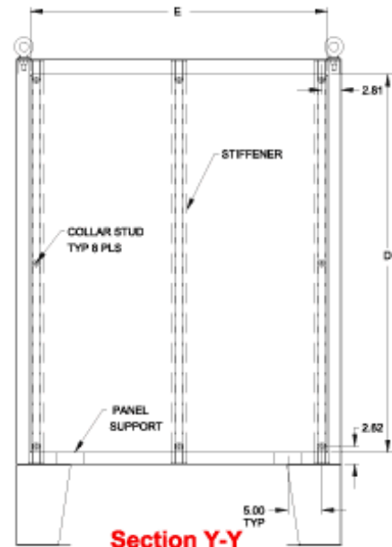
Section Y-Y
