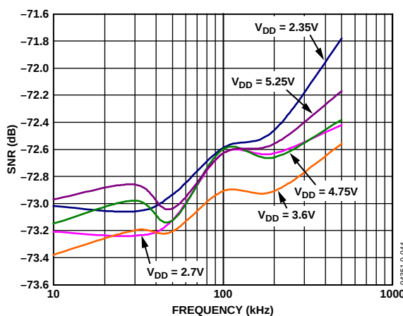
Figure 13. AD7922 SNR vs. Input Frequency at 1 MSPS
