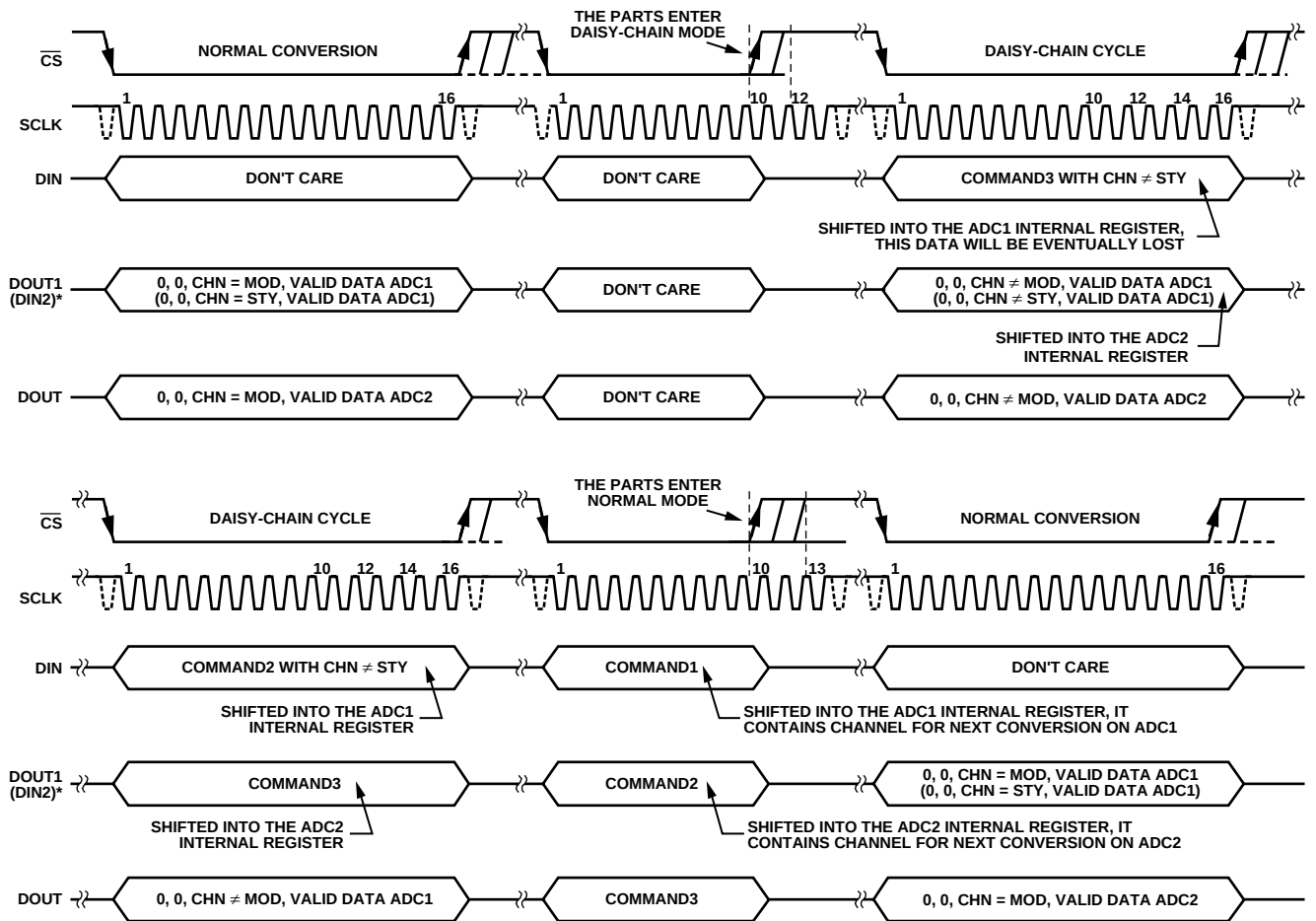
Figure 35. Daisy-Chain Diagrams—II
