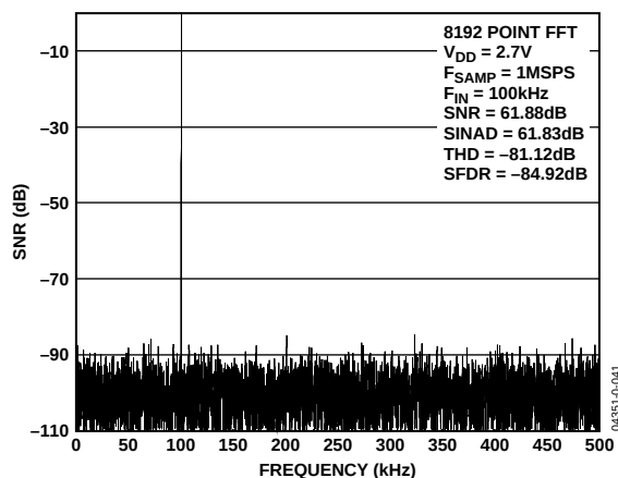
Figure 11. AD7912 Dynamic Performance at 1 MSPS
