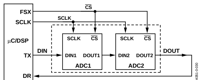
Figure 33. AD7912/AD7922 Connected in Daisy Chain
