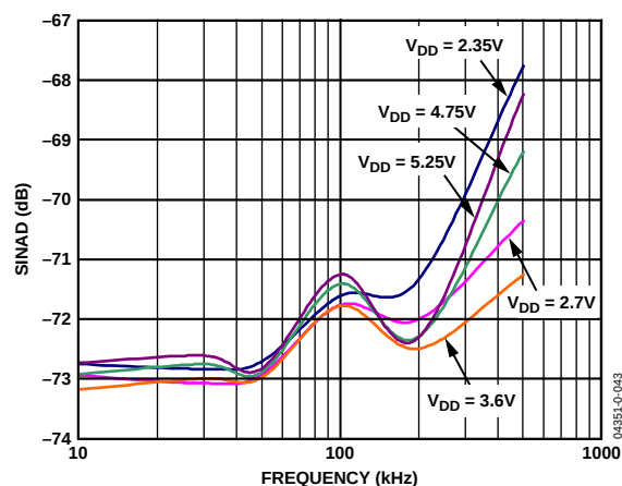
Figure 12. AD7922 SINAD vs. Input Frequency at 1 MSPS
