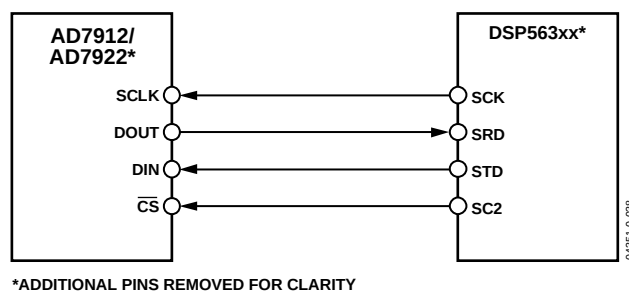
Figure 41. Interfacing to the DSP563xx
