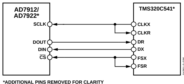
Figure 39. Interfacing to the TMS320C541
