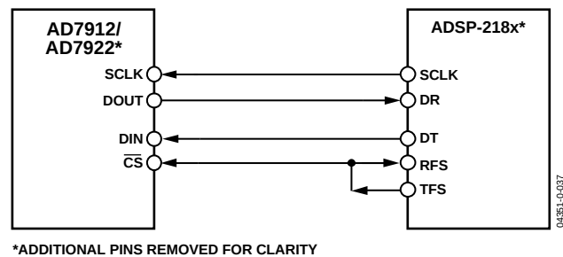
Figure 40. Interfacing to the ADSP-218x
