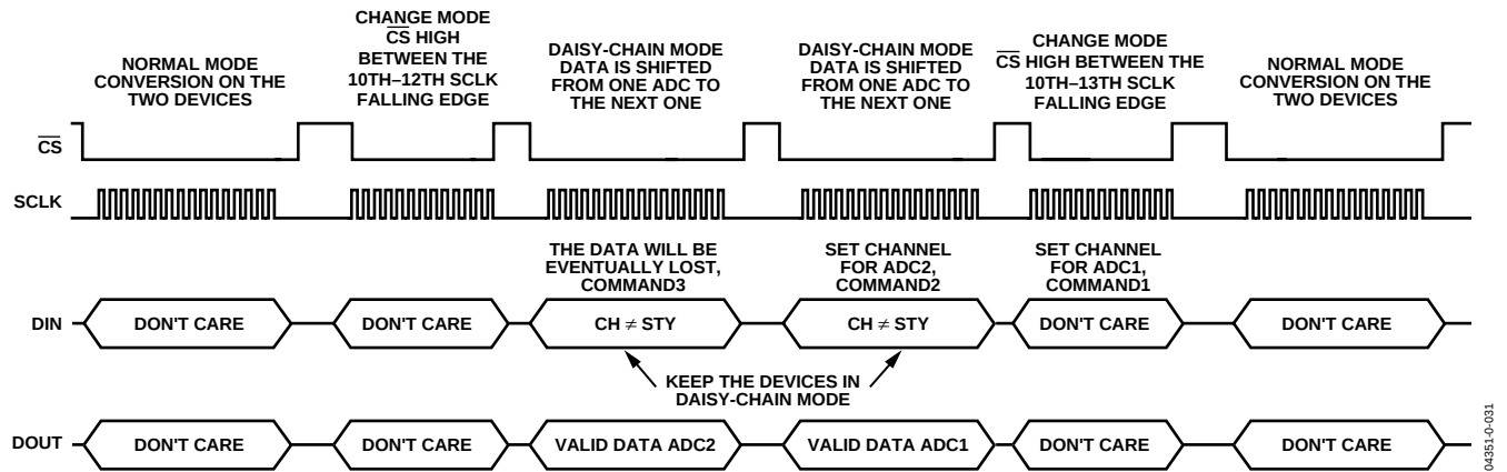
Figure 34. Daisy-Chain Diagrams—I
