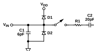
Figure 23. Equivalent Analog Input Circuit
