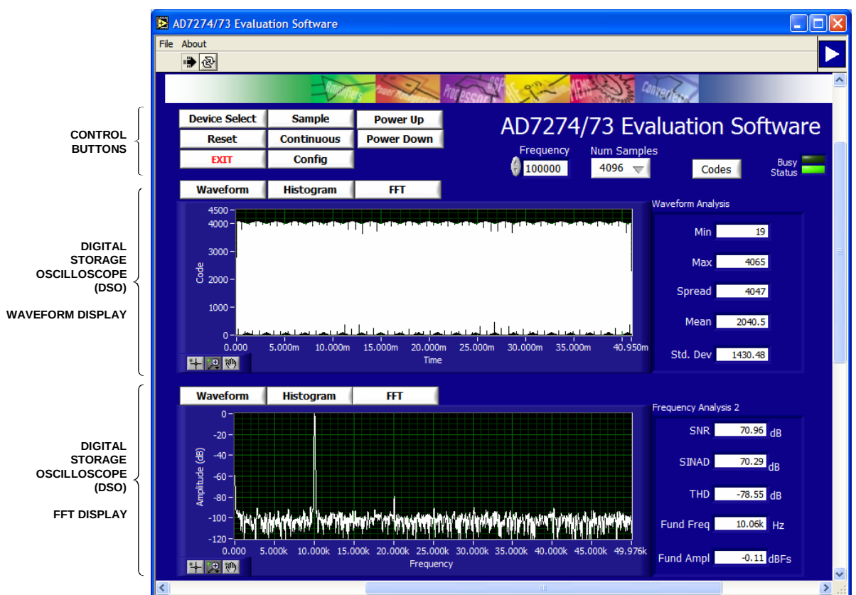
Figure 4. AD7273/AD7274 Main Window
