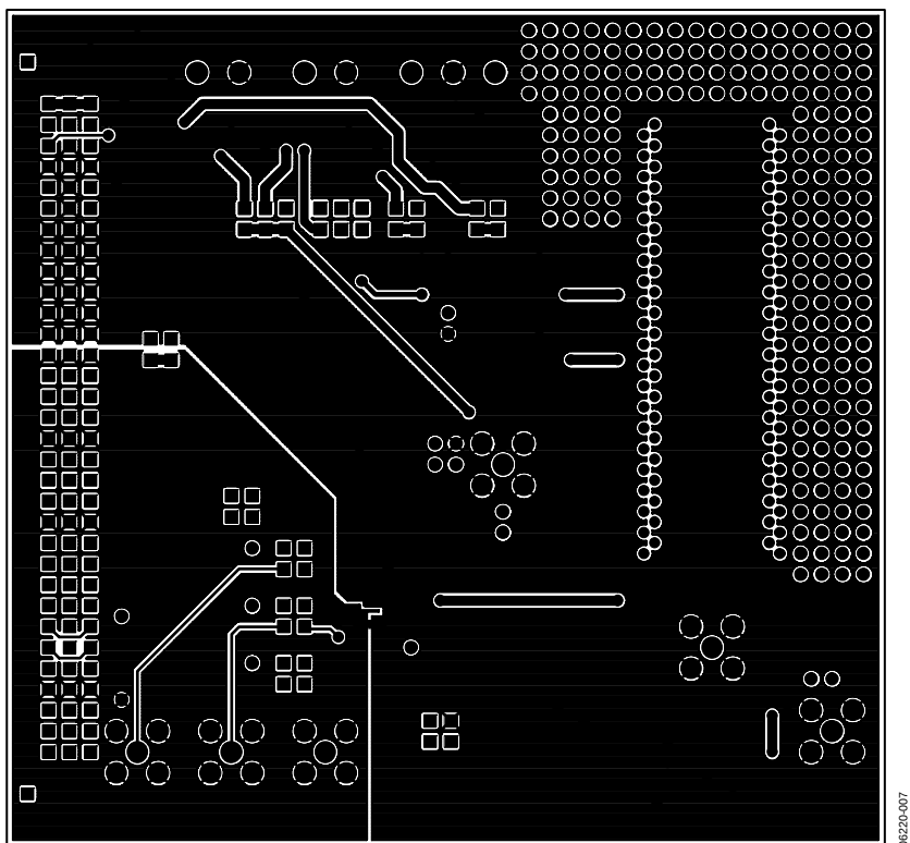
Figure 7. Top View, Solder Side
