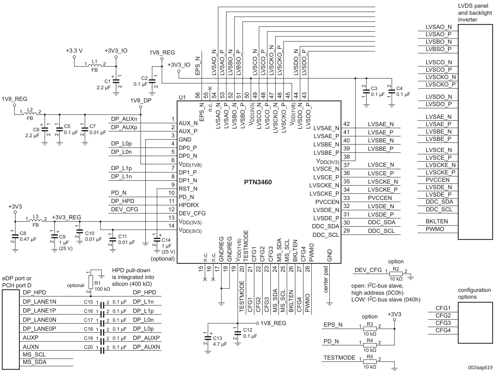
Fig 5. Application diagram
