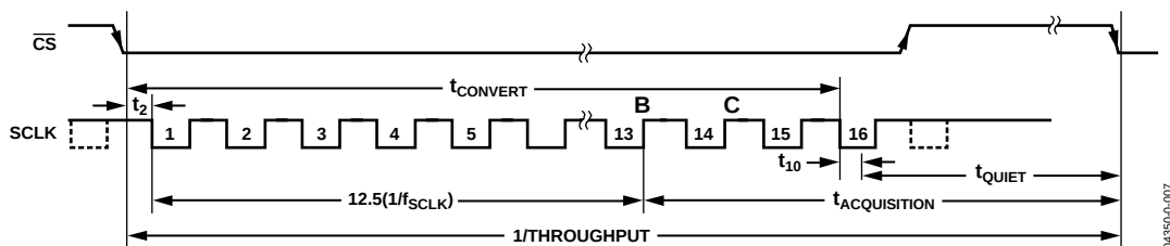
Figure 6. AD7921 Serial Interface Timing Diagram
