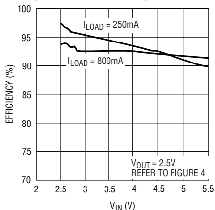
OUT2 Efficiency vs V_{IN} (Pulse Skipping Mode)
