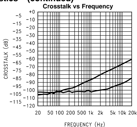
V_{DD} = 3V ; LLS, RLS; P_O = 200mW ; R_L = 8\Omega ; Mode 7; 0db Gain; 3D off Top-Left to Right; Bot-Right to Left Figure 21.
