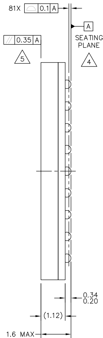
SIDE VIEW
