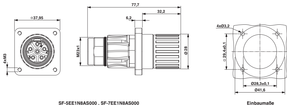
SF-5EE1N8AS000, SF-7EE1N8AS000
