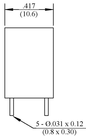
Relay 4 Pin
