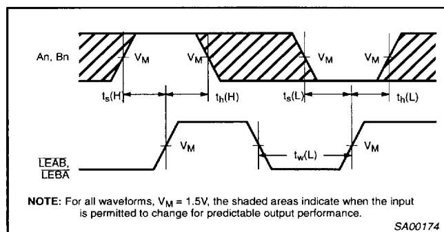
Waveform 3. Data Setup and Hold Times And Latch Enable Pulse Width
