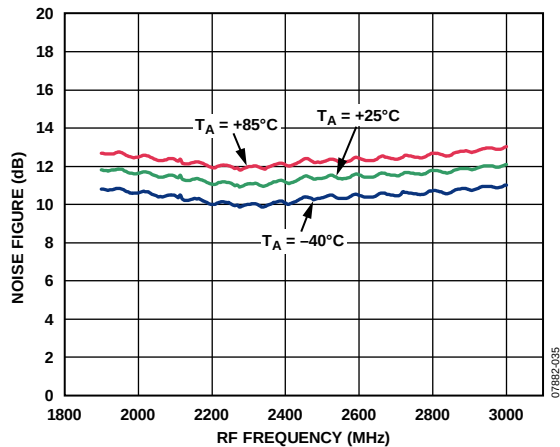
Figure 35. SSB Noise Figure vs. RF Frequency ( V_{SET} = 2.0\text{ V} )
