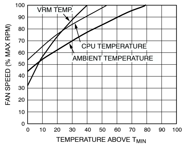
Figure 63. T_{\text{RANGE}} and % Fan Speed Slopes for VRM, Ambient, and CPU Temperature Channels
