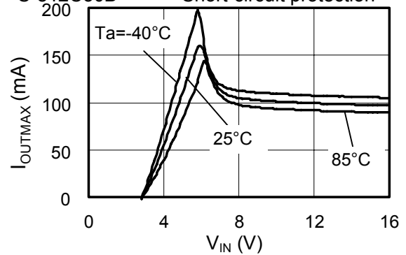
S-812C30B Short-circuit protection
