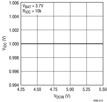
IDC Pin Voltage vs V_{\text{DCIN}} (Constant-Current Mode)
