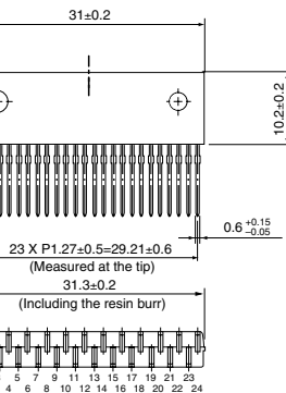
Forming No.2452
