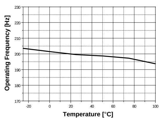
Figure 8. Operating Frequency vs. Temperature
