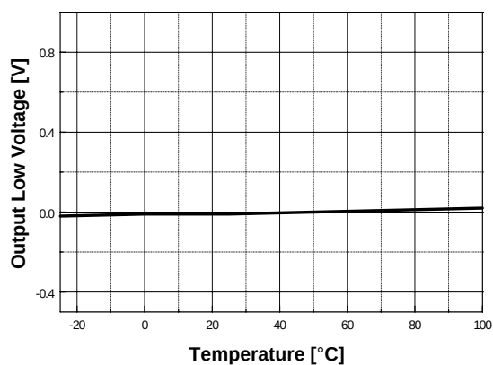
Figure 12. Output Low Voltage vs. Temperature
