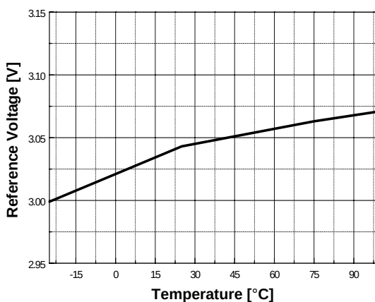
Figure 6. Reference Voltage vs. Temperature
