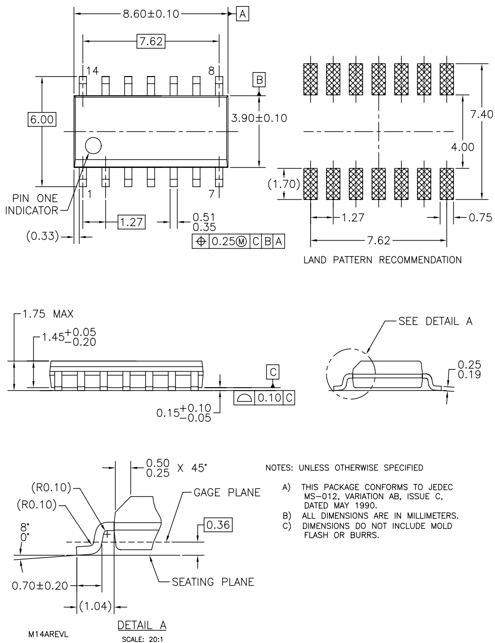
Figure 14. 14-Lead Small Outline Package (SOP)
