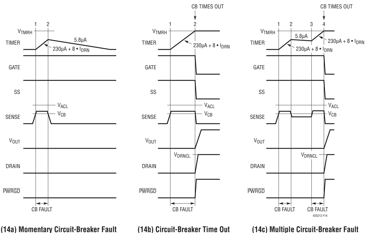
Figure 14. Circuit-Breaker Timing Behavior (All Waveforms Are Referenced to V_{FF} )
