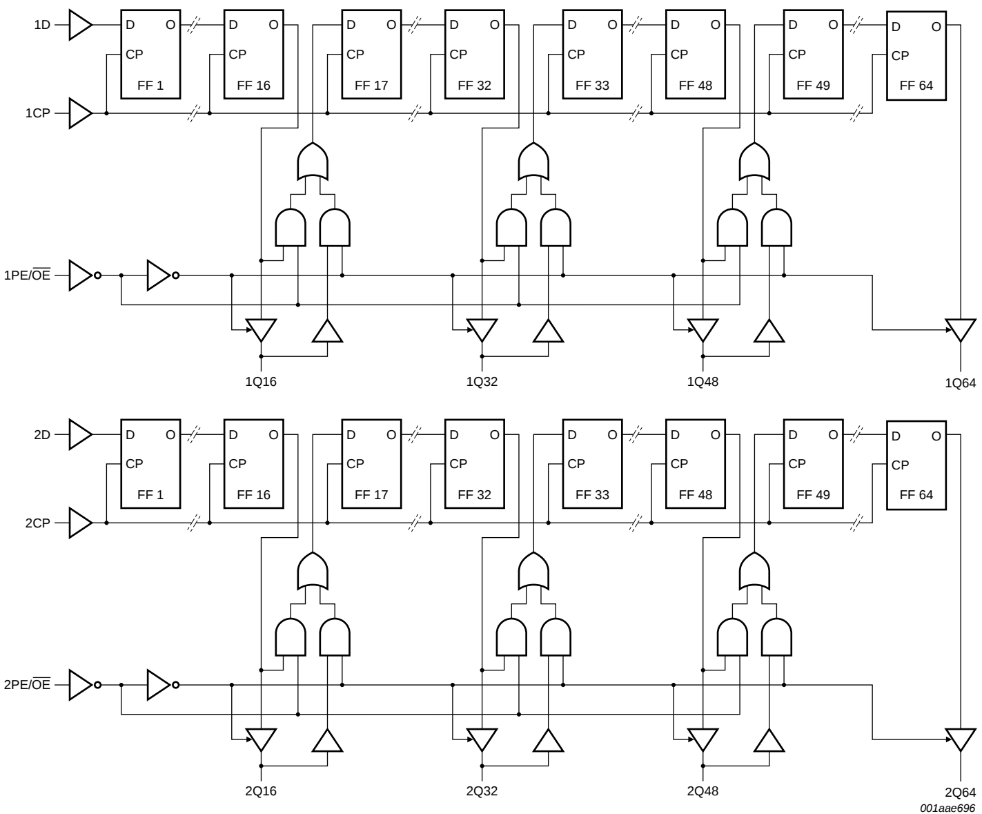
Fig 2. Logic diagram
