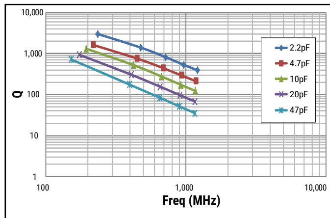
Q vs. Frequency 0603
