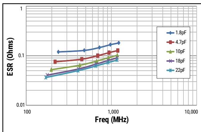
ESR vs. Frequency 0402
