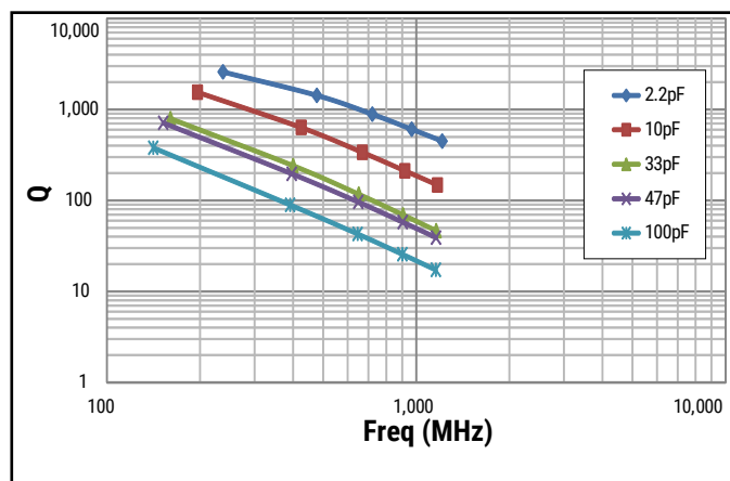
Q vs. Frequency 0805
