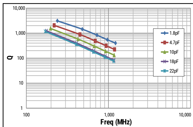
Q vs. Frequency 0402
