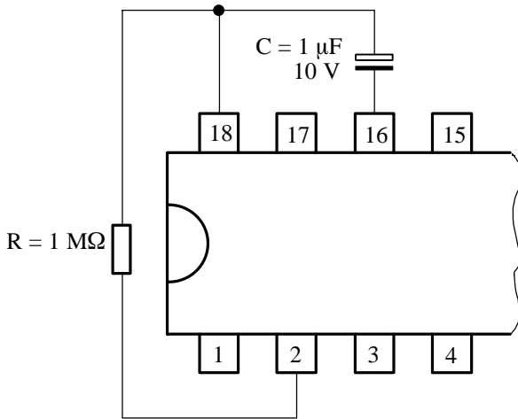
Figure 7. Operation delay
