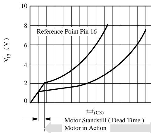
Figure 14. Soft-start function
