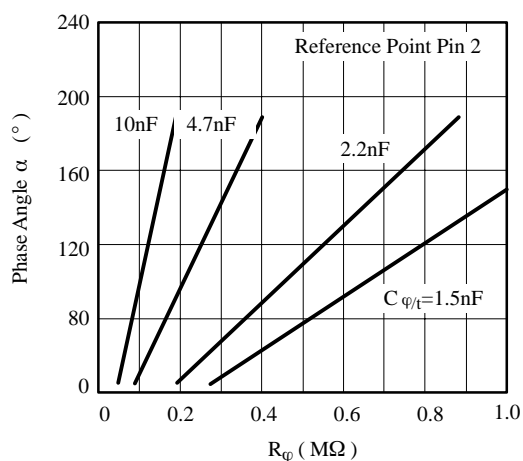
Figure 9. Ramp control
