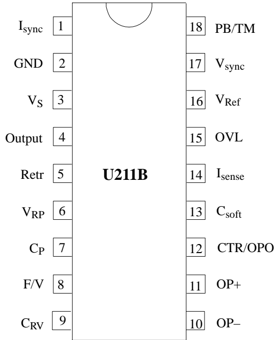
Figure 3. Pinning DIP18
