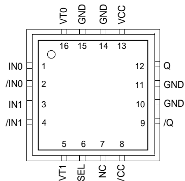
16-Pin MLF™
