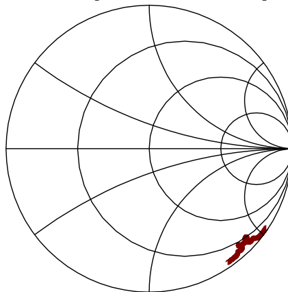
S22 (28.2-44.2 MHz)
