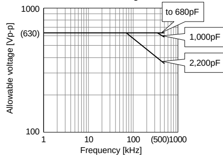
U2J char., Rated Voltage: DC3.15kV
