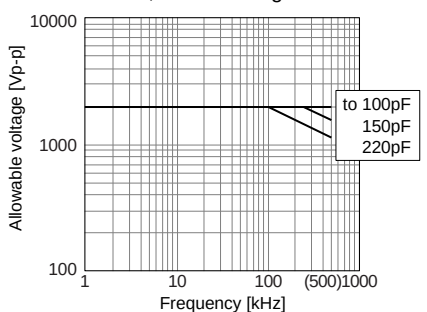
U2J char., Rated Voltage: DC2kV
