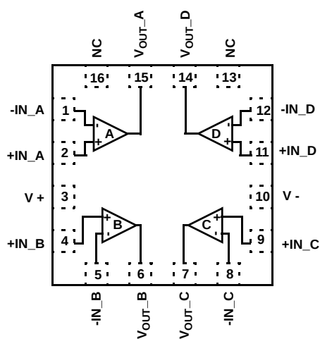
ISL28407 (16 LD QFN) TOP VIEW
