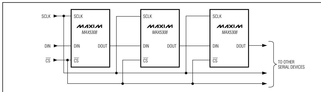
Figure 5. Daisy-Chaining MAX5308s
