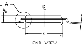
END VIEW
