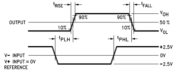
Figure 3. Propagation Delay
