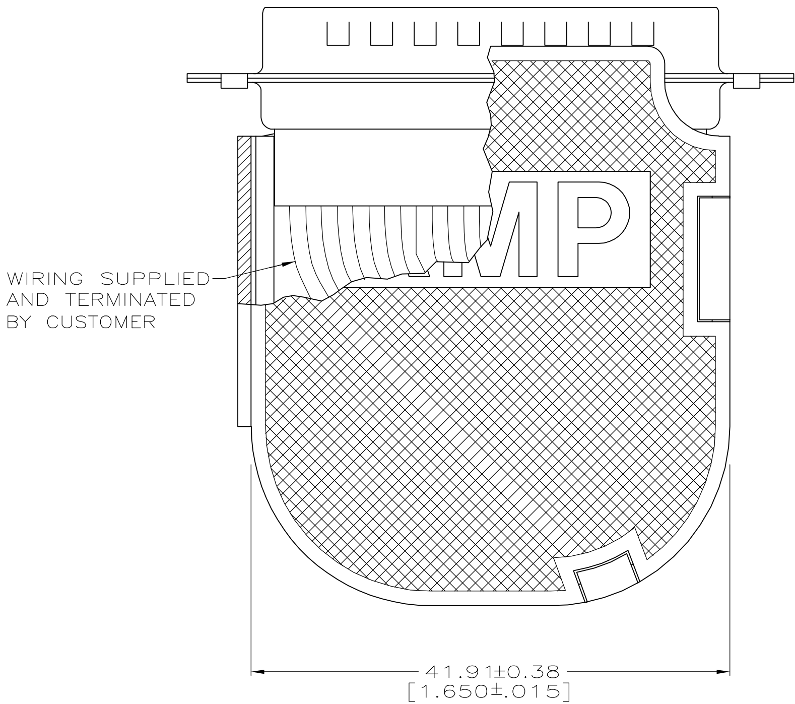
ASSEMBLED VIEW
