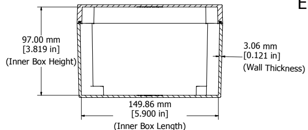
SECTION R-R Side View of Assembly
