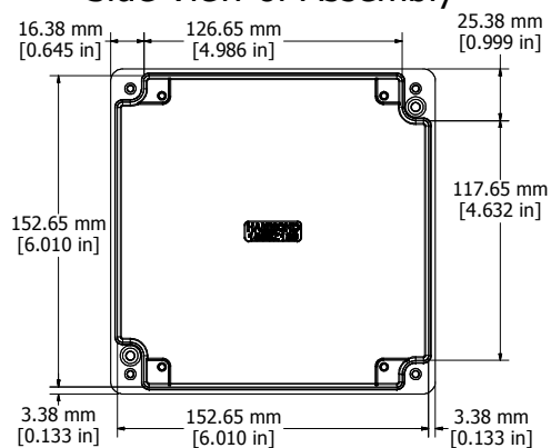
Top View Looking Inside Box
