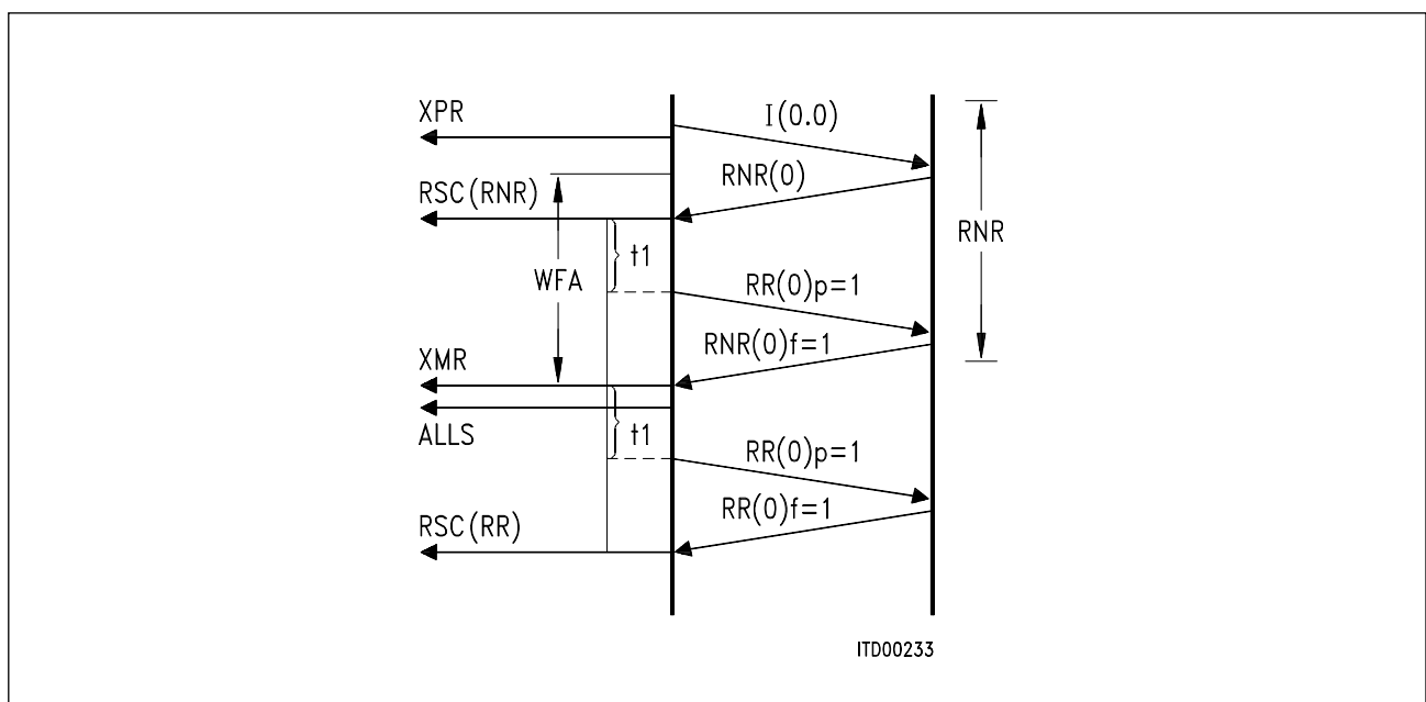
Figure 24 Flow Control/Transmission
