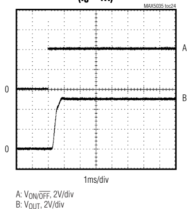
MAX5035DASA STARTUP WAVEFORM ( I_Q = 1A )
