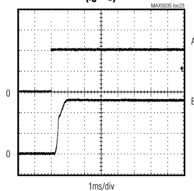
MAX5035DASA STARTUP WAVEFORM ( I_Q = 0 )
