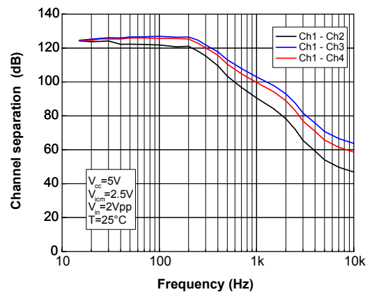
Figure 37. Channel separation on TSU104
